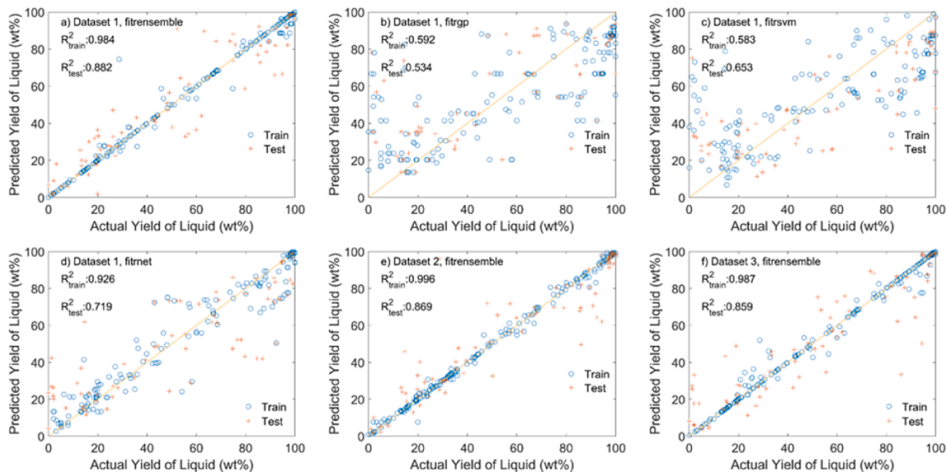
Fig. 4. Scatter plots of the pairs of input variables and responses with different algorithms and datasets: (a) Dataset 1 with fitrensemble, (b) Dataset 1 with fitrgp, (c) Dataset 1 with fitrsvm, (d) Dataset 1 with fitnet, (e) Dataset 2 with fitrensemble, and (f) Dataset 3 with fitrensemble.
